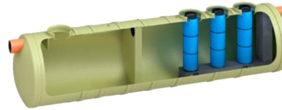
Central Oil Separators
